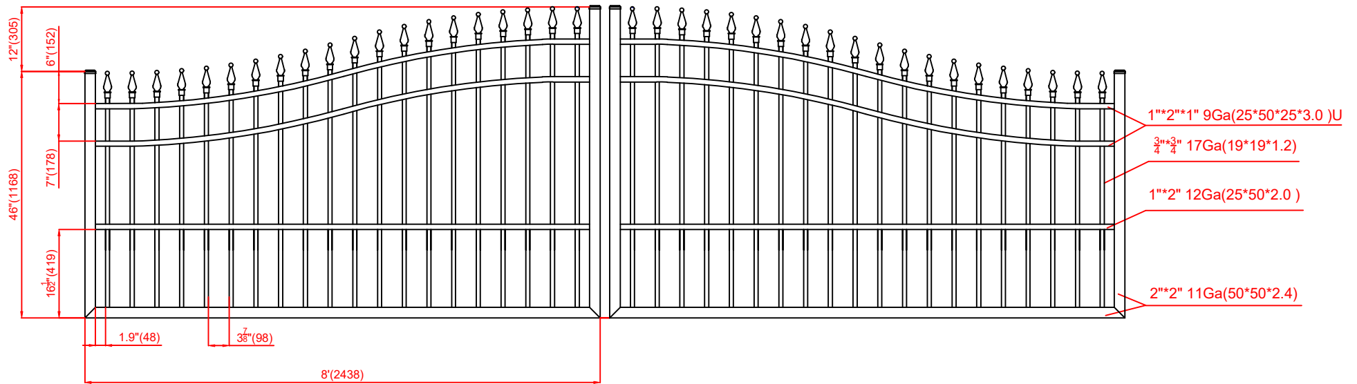
GATE-16' x 4' to 5' DDE-JF-ALUMINUM
